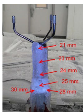
Figure 6. New sensor design was operative throughout the test period with the freezing rain test profile (Table 3). In this test, the body heating was inactivated.
