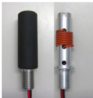
Figure 5. On left, the dummy scale model of a transducer stack had a wire heater embedded to a rubber. On right, the heating variation options of the dummy transducer stack were “centered”, “whole”, and “edge”.
