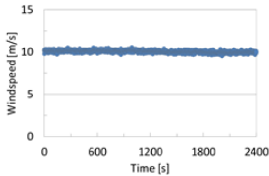
Figure 8. The WMT700 Ultrasonic Wind sensor with the new modified transducer stacks was operative throughout the icing test period of 40 minutes performed in the icing wind tunnel of the KAIT.
