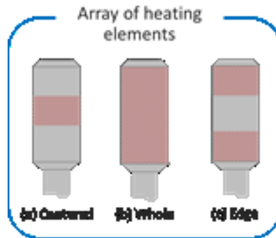
Figure 5. On left, the dummy scale model of a transducer stack had a wire heater embedded to a rubber. On right, the heating variation options of the dummy transducer stack were “centered”, “whole”, and “edge”.
