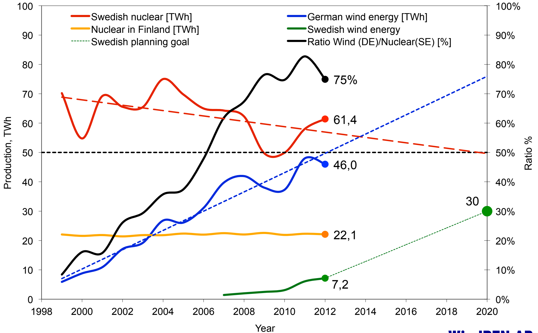
Annual German & Swedish wind energy - Swedish and Finnish nuclear energy production
