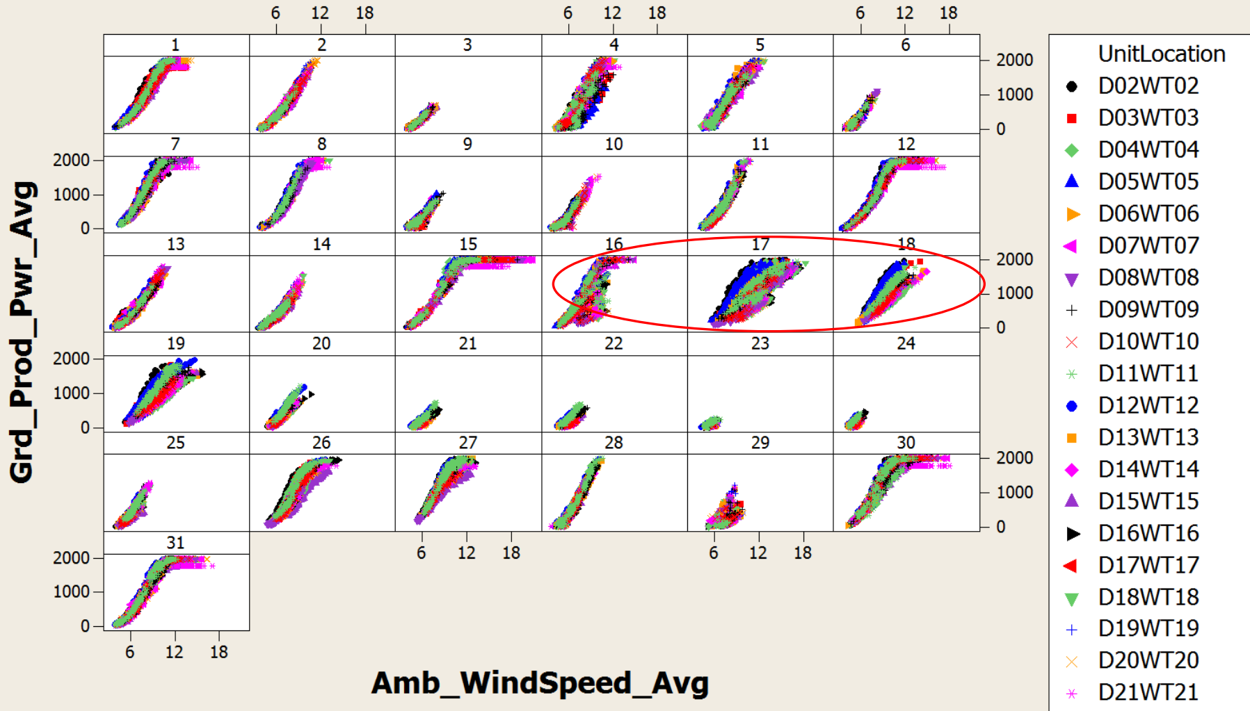
Scatterplot of Grd_Prod_Pwr_Avg vs Amb_WindSpeed_Avg
